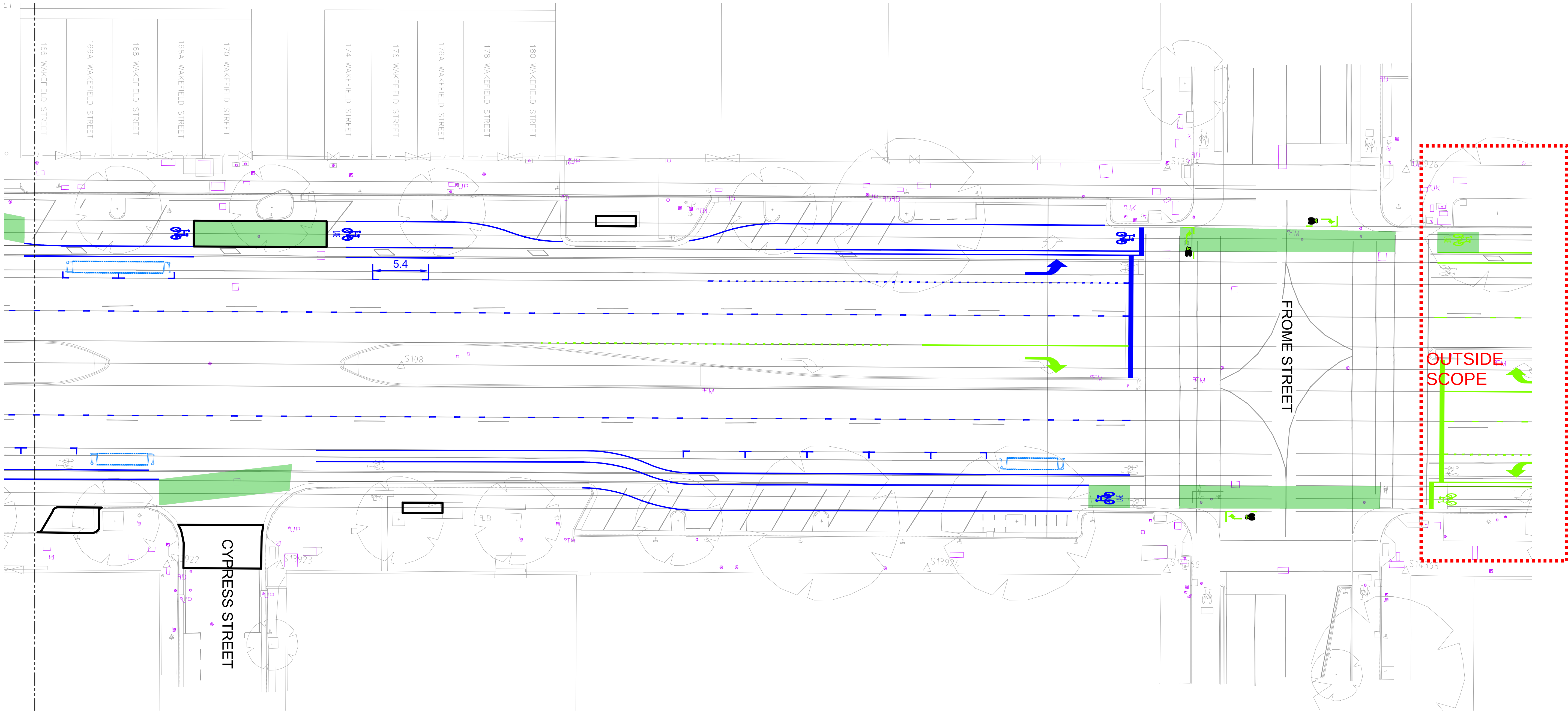
LAYOUT 5 SCALE 1:200
