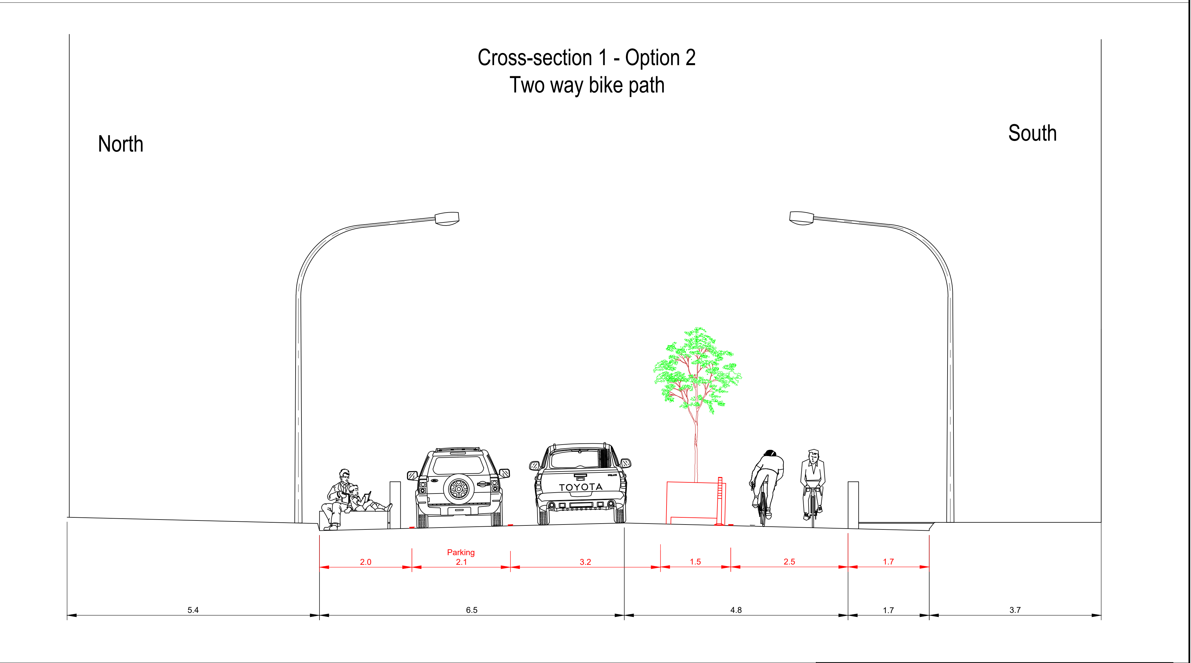
Cross-section 1:50
